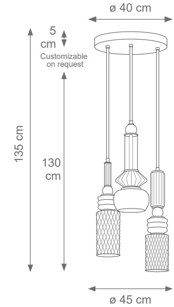
Lolite Chandelier Code F808229 Type 3 lights electrification x Max 28W E14 CE Size: cm. 135 h x 45 ø - 9 kg
