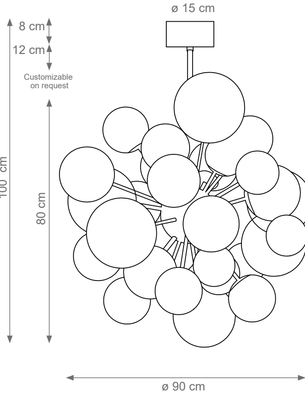
Lady V Chandelier Code: F807905 Type 32 lights electrification x Max 28W E14 CE Size: cm. 80 h x 90 ø - 26 Kg
