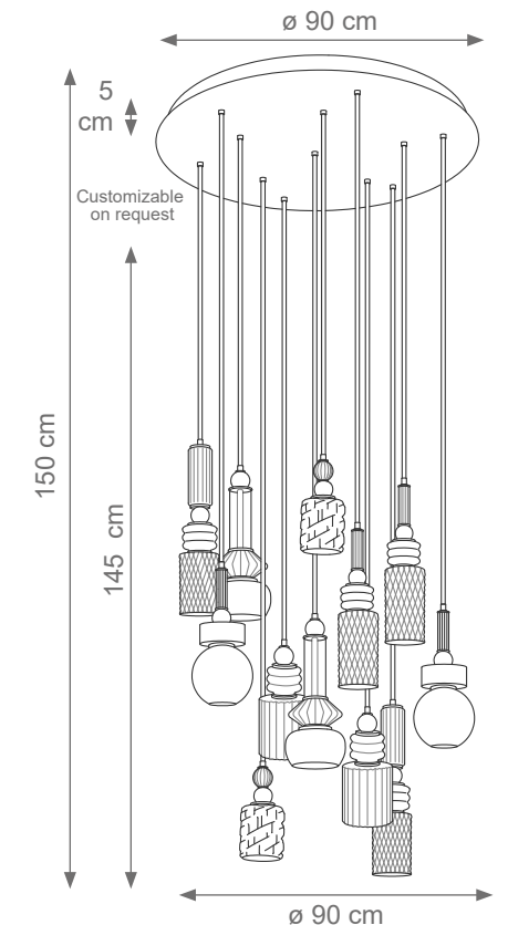
Gran Lolite Chandelier Code F808199 Type 12 lights electrification x Max 28W E14 CE Size: cm. 150 h x 90 ø - 35 kg
