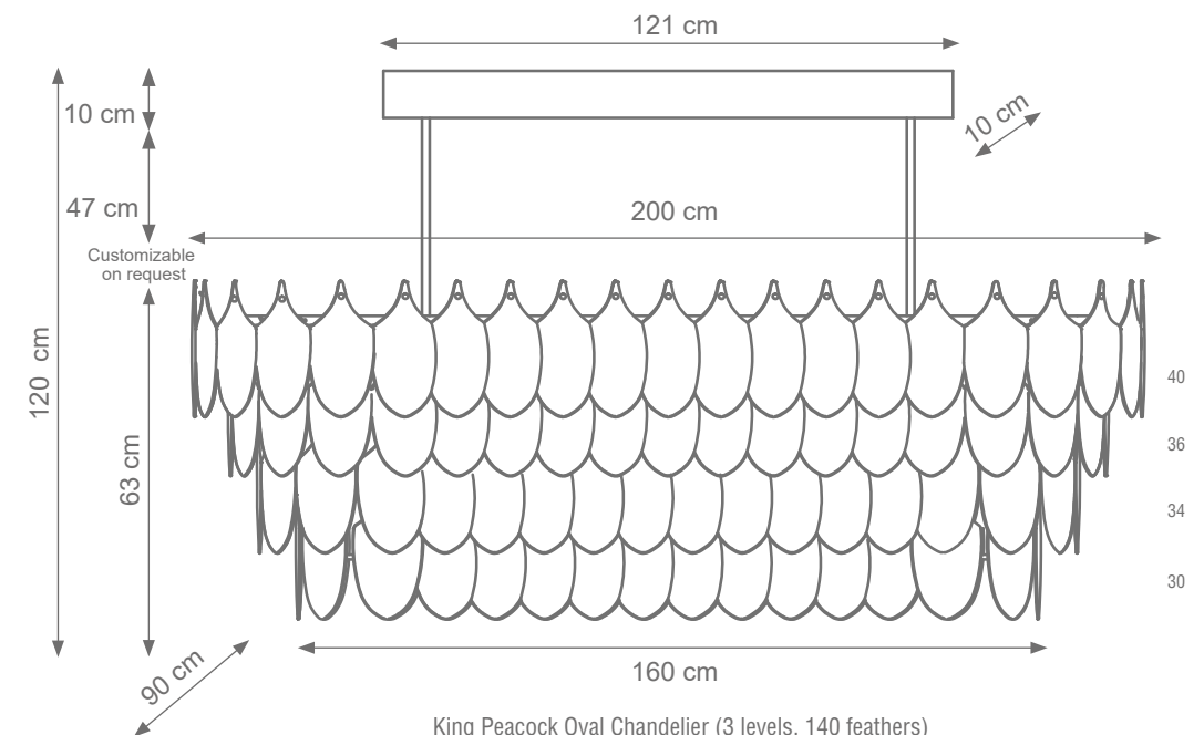
King Peacock Oval Chandelier (3 levels, 140 feathers) Code: F807562 Type 24 lights electrification x Max 28W E14 CE Size: cm. 63 h x 200 l x 90 w - 98 kg
