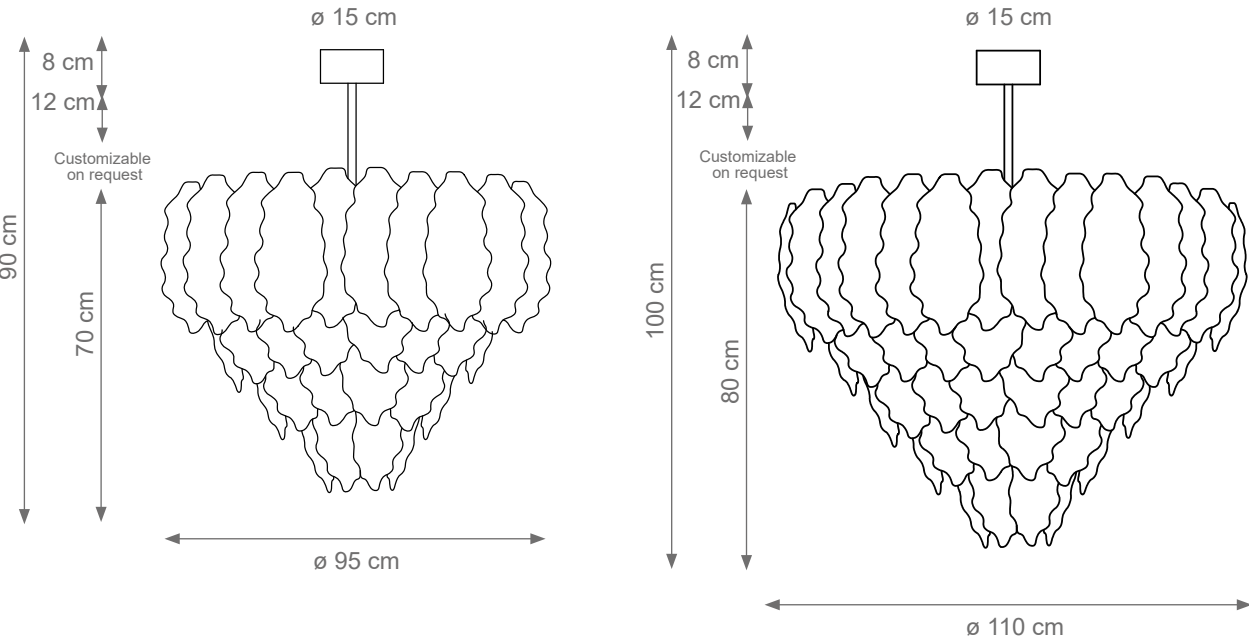
Medium Kelly Chandelier Code: F808225 Type 9 lights electrification x Max 28W E14 CE Size: cm. 70 h x 95 ø - 70 kg
