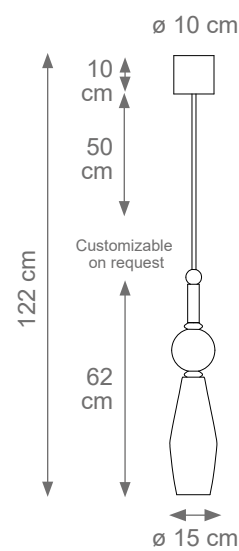
Lola Pendant Light Code F707340 Type 1 light electrification x Max 28W E14 CE Size: cm. 62 h x 15 ø - 3 kg
