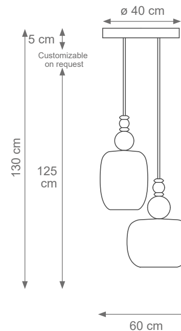
Icons '80 Chandelier Code: F807918 Type 2 lights electrification x Max 28W E14 CE Size: cm. 130 h x 60 ø - 16 kg
