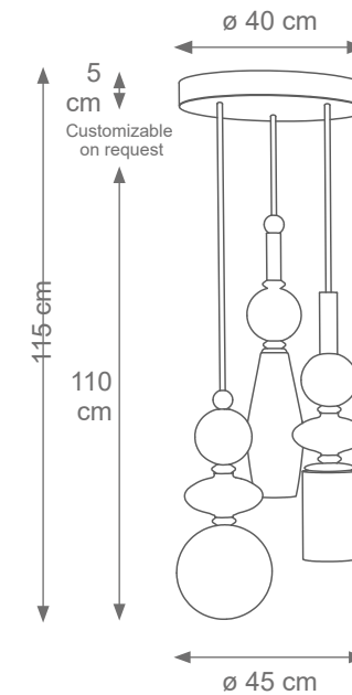
Divas Chandelier Code F807767 Type 3 lights electrification x Max 28W E14 CE Size: cm. 115 h x 45 ø - 15 kg
