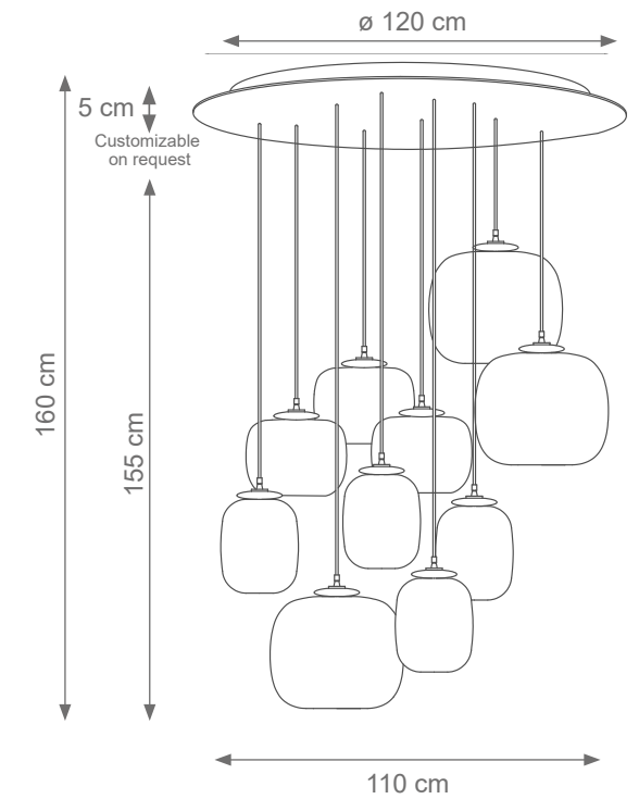
Grand Salento Chandelier Code: F808195 Type 10 lights electrification x Max 28W E14 CE Size: cm. 160 h x 120 ø - 72 kg
