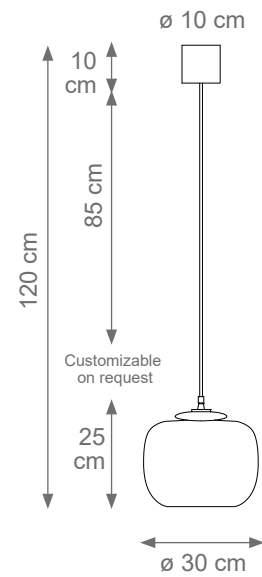
Specchia Pendant Light Code: F808000 Type 1 light electrification x Max 28W E14 CE Size: cm. 25 h x 30 ø - 3 kg
