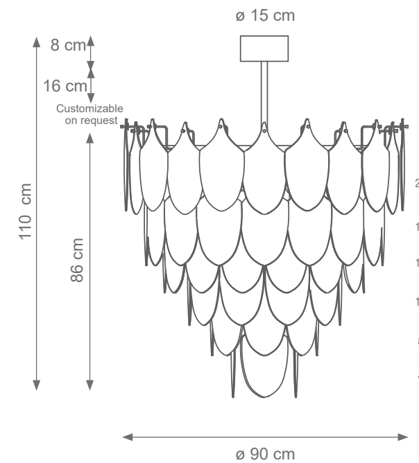
Medium Peacock Chandelier (6 levels, 72 feathers) Code: F807277 Type 12 lights electrification x Max 28W E14 CE Size: cm. 86 h x 90 ø - 54 kg
