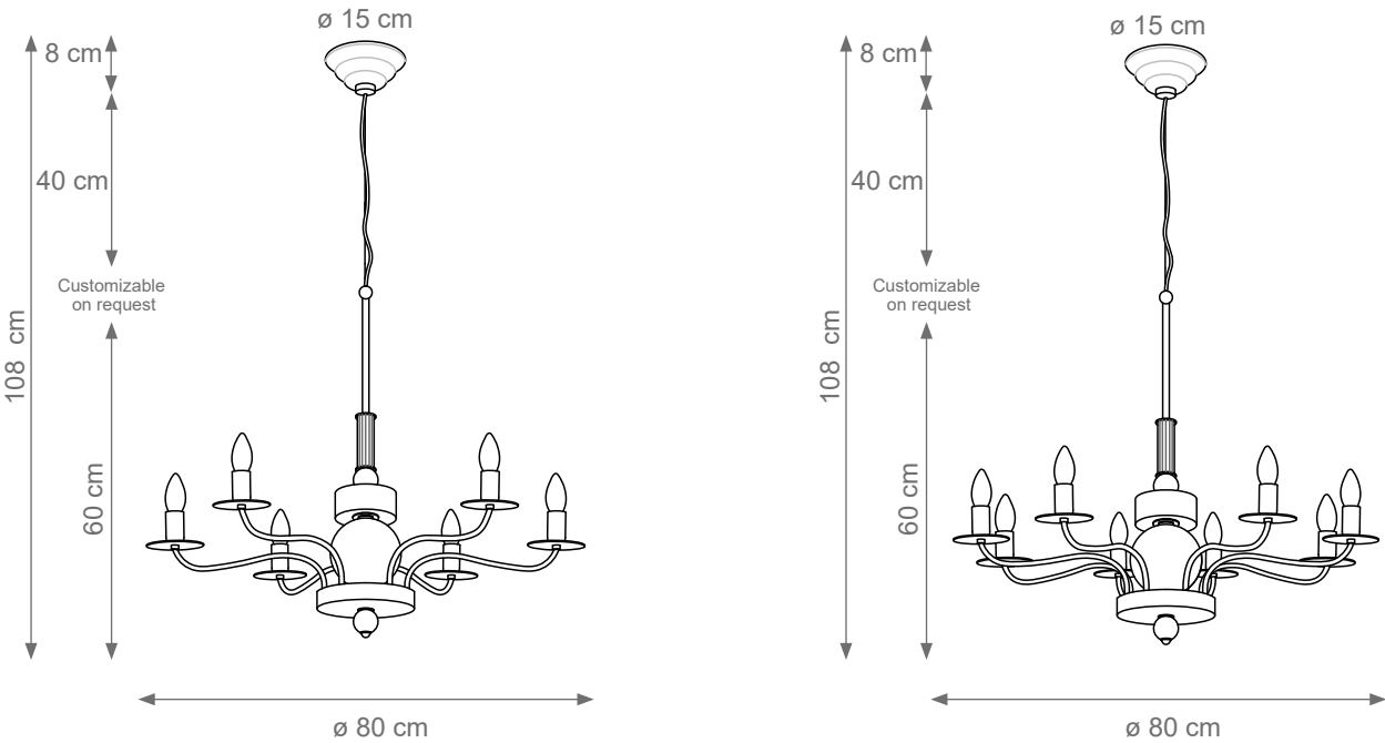
Etienne Chandelier Code: B808119 Type 6 lights electrification x Max 28W E14 CE Size: cm. 60 h x 80 ø - 4,5 Kg
