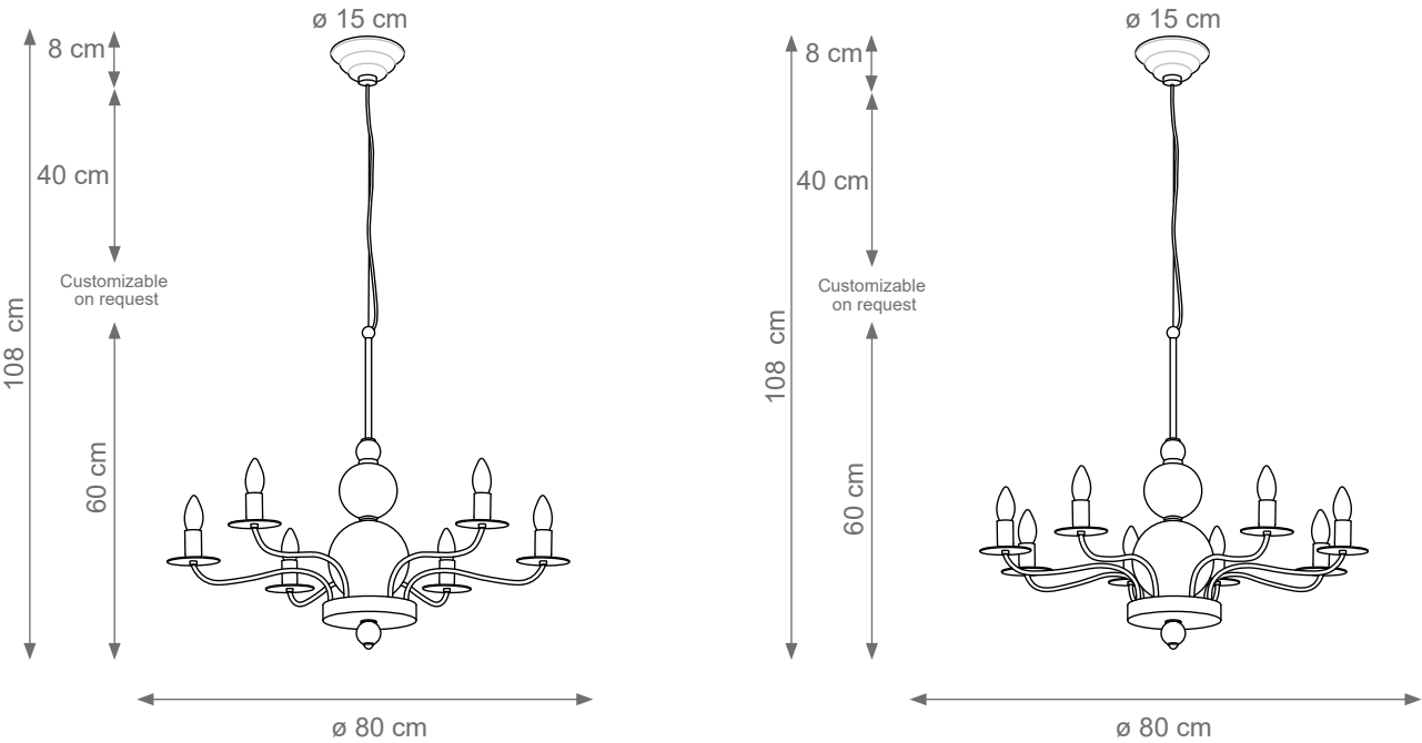
Lady V Chandelier Code: B808125 Type 6 lights electrification x Max 28W E14 CE Size: cm. 60 h x 80 ø - 4,5 Kg
