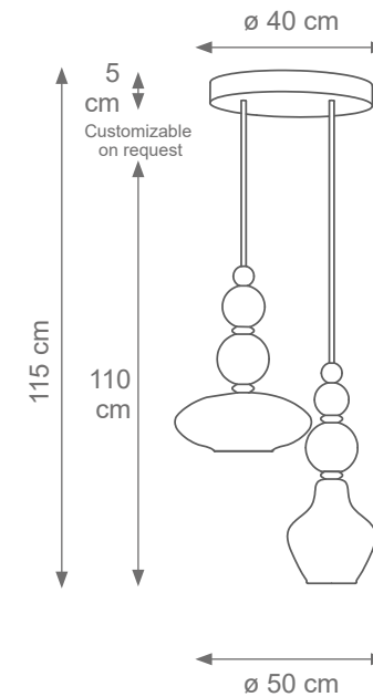
Divas Chandelier Code F807766 Type 2 lights electrification x Max 28W E14 CE Size: cm. 115 h x 50 ø - 12 kg
