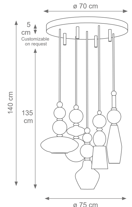
Divas Chandelier Code F807595 Type 5 lights electrification x Max 28W E14 CE Size: cm. 140 h x 75 ø - 23 kg
