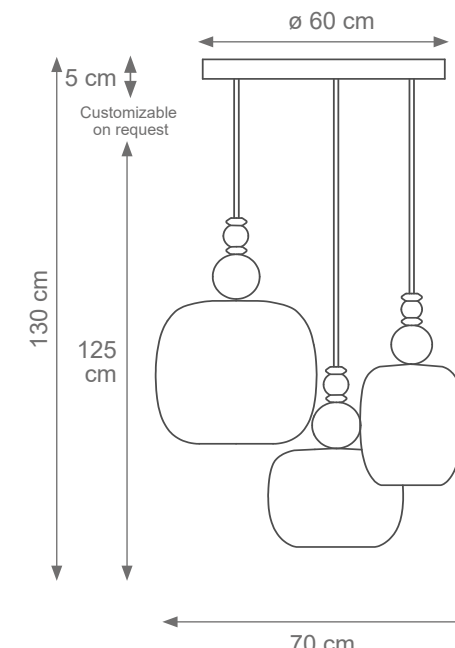
Icons '80 Chandelier Code: F807919 Type 3 lights electrification x Max 28W E14 CE Size: cm. 130 h x 70 ø - 22 kg
