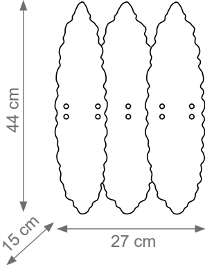
Cher Wall Light Code F808212 Type 2 lights electrification x Max 28W G9 CE Size: cm. 44 h x 27 l x 15 w - 3 kg
