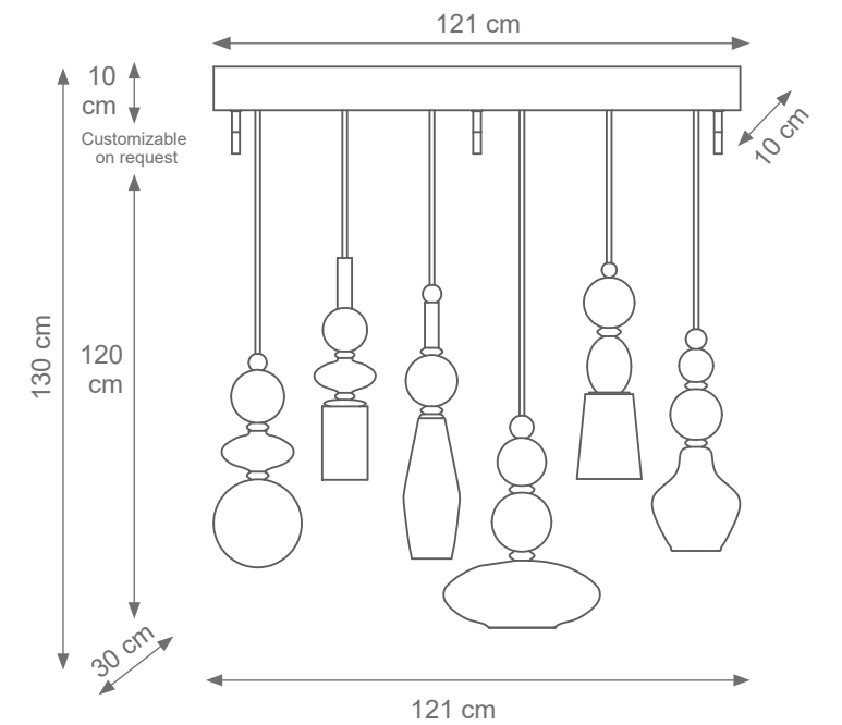
Long Divas Chandelier Code F807670 Type 6 lights electrification x Max 28W E14 CE Size: cm. 130 h x 121 l x 30 w - 25 kg
