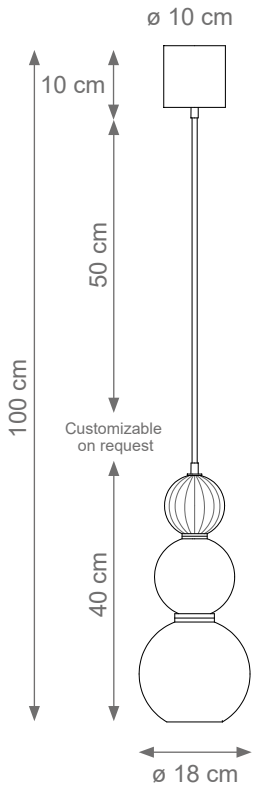
Lady V Pendant Light Code: F807936 Type 1 light electrification x Max 28W E14 CE Size: cm. 40 h x 18 ø - 3 Kg
