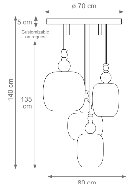
Icons '80 Chandelier Code: F808242 Type 4 lights electrification x Max 28W E14 CE Size: cm. 140 h x 80 ø - 27 kg
