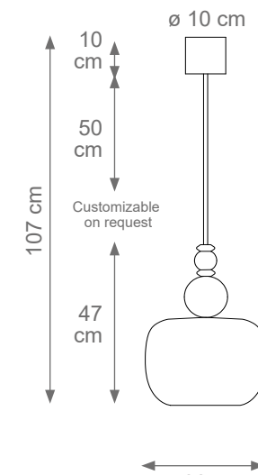
Farrah Medium Pendant Light Code: F807353 Type 1 light electrification x Max 28W E14 CE Size: cm. 47 h x 30 ø - 5 kg
