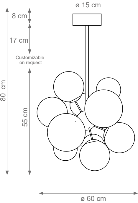
Small Lady V Chandelier Code: F807840 Type 12 lights electrification x Max 28W E14 CE Size: cm. 55 h x 60 ø - 16 Kg
